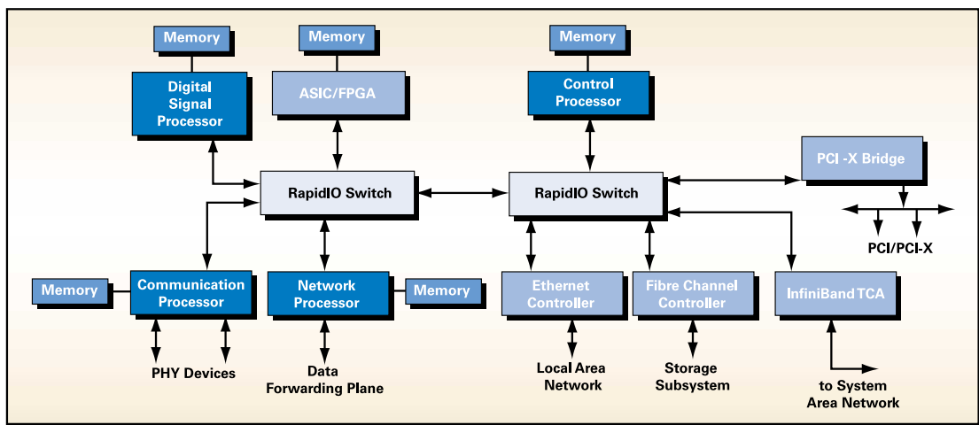
RapidIO Architecture is a Point-to-Point Interconnect that Bridges to Existing Systems and Networks
